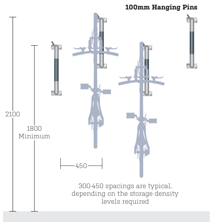
Front View Vertical Bicycle Storage
