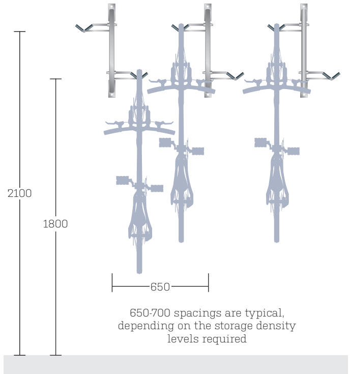
Front View Vertical Bicycle Storage 2 bike capacity
